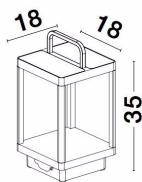
Maßskizze BALI M LED
